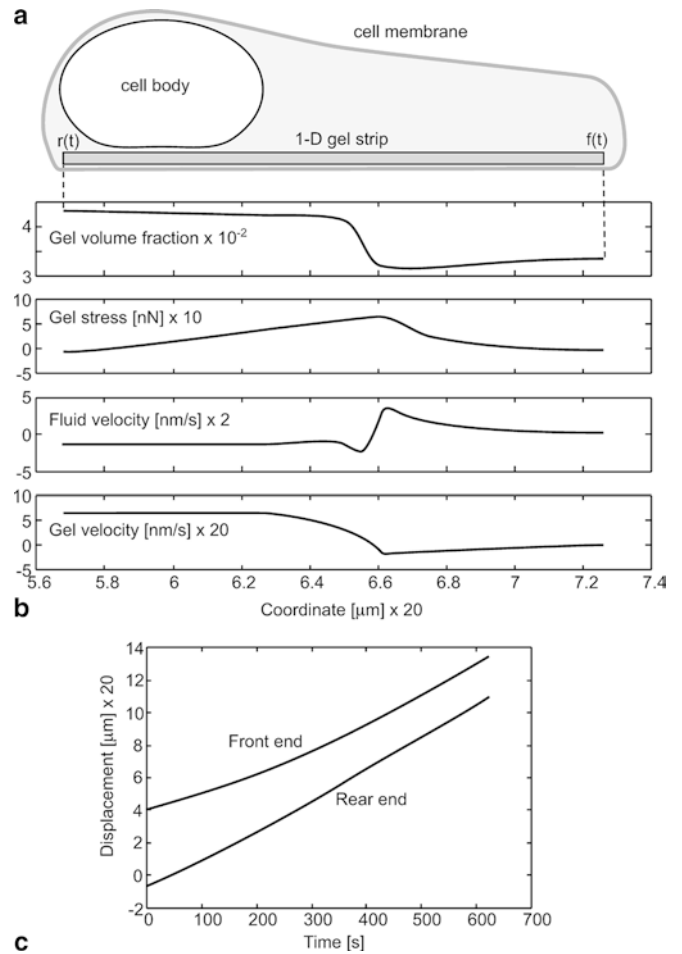
Fig. 3 a Side view of a crawling nematode sperm showing the gel strip model. (b) Asymptotically stable stationary distributions of the polymer volume fraction, stress, and velocity and of the fluid velocity from the rear to the front of the cell. (c) Trajectories of the front and rear ends of the 1-D cytogel strip. Over a few hundred seconds the cell length regulates to a constant value
